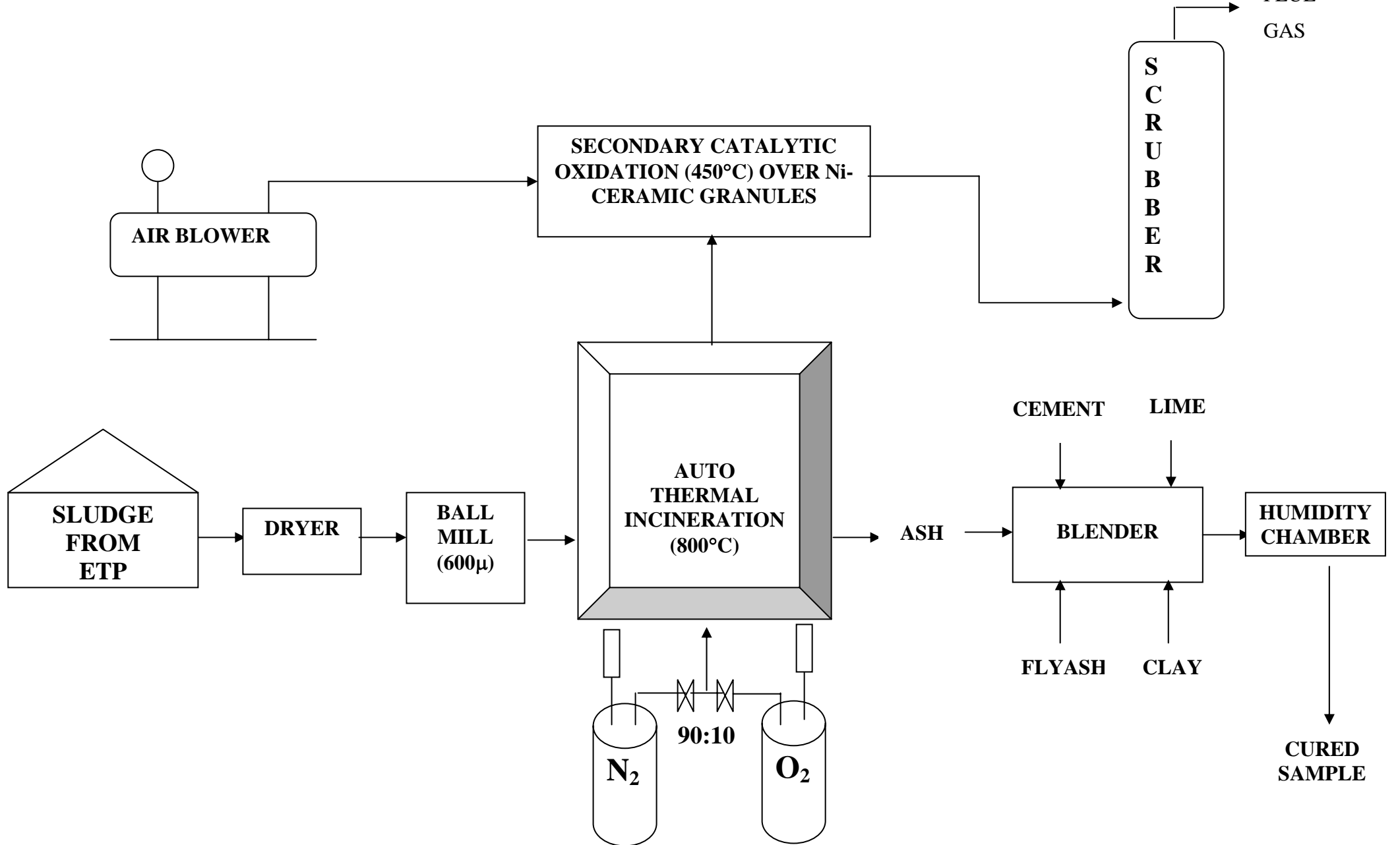
Figure 1. Auto Thermal Incineration and Solidification/Stabilization system for sludge discharged from a leather manufacturing industry
