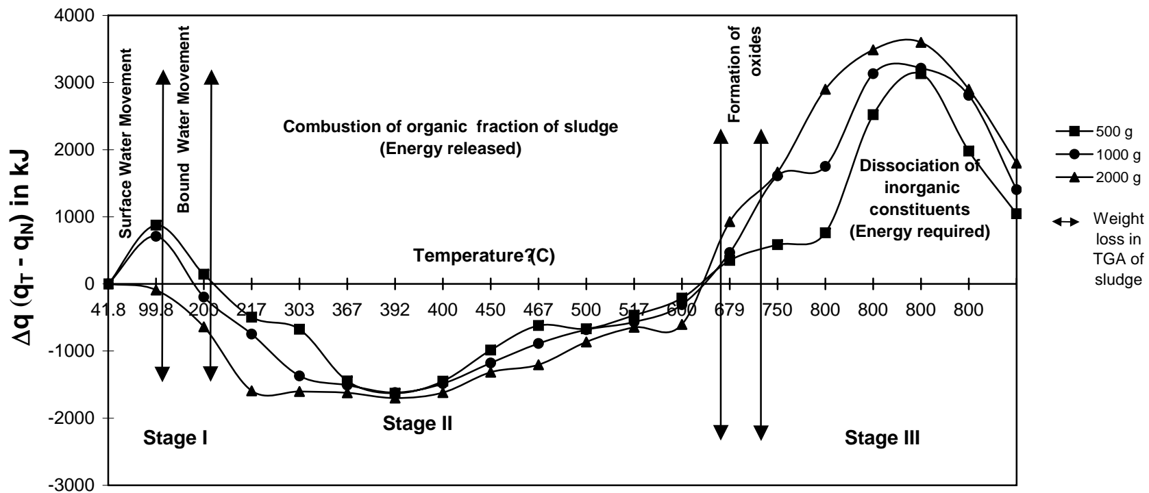
Figure 2. Net energy change ( \Delta q ) with respect to furnace temperature for various loading rate of sludge correlated with TGA
