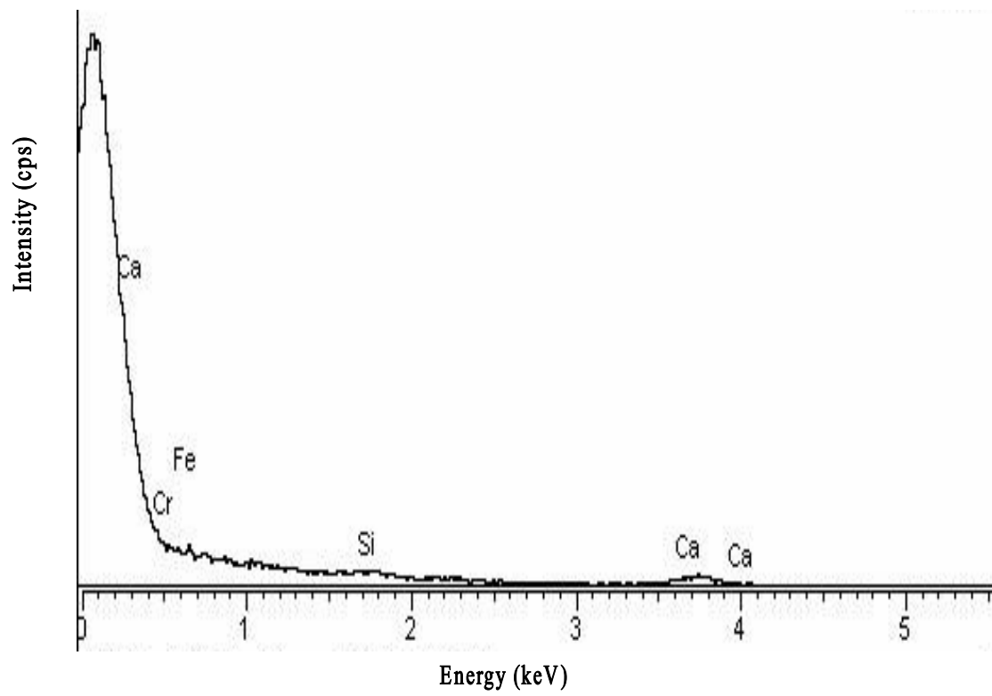
Figure 7. EDX microanalysis of the solidified specimen
